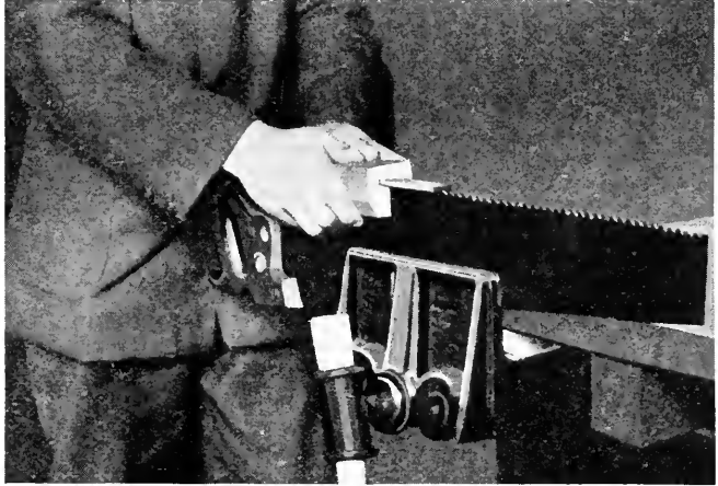
Fig. 24. Jointing a Saw.
